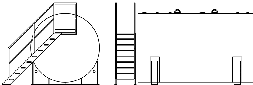
End Mounted Stairway Parallel to End
