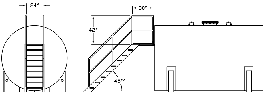
Straight-on End Mounted Stairway
