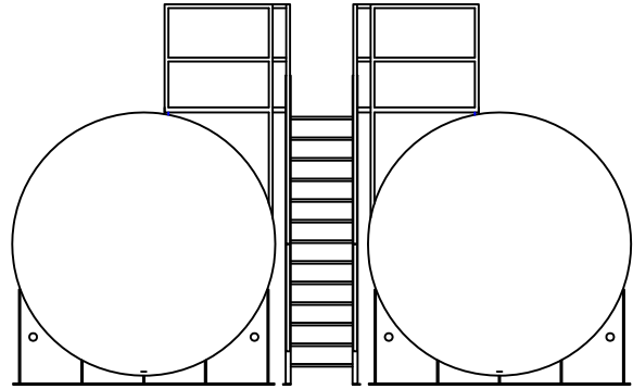
T-Box Stairway for in-between two or more tanks for top of tank access
