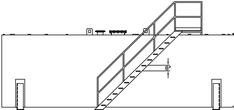
Side Mounted Stairway Parallel to Tank for top of tank access
